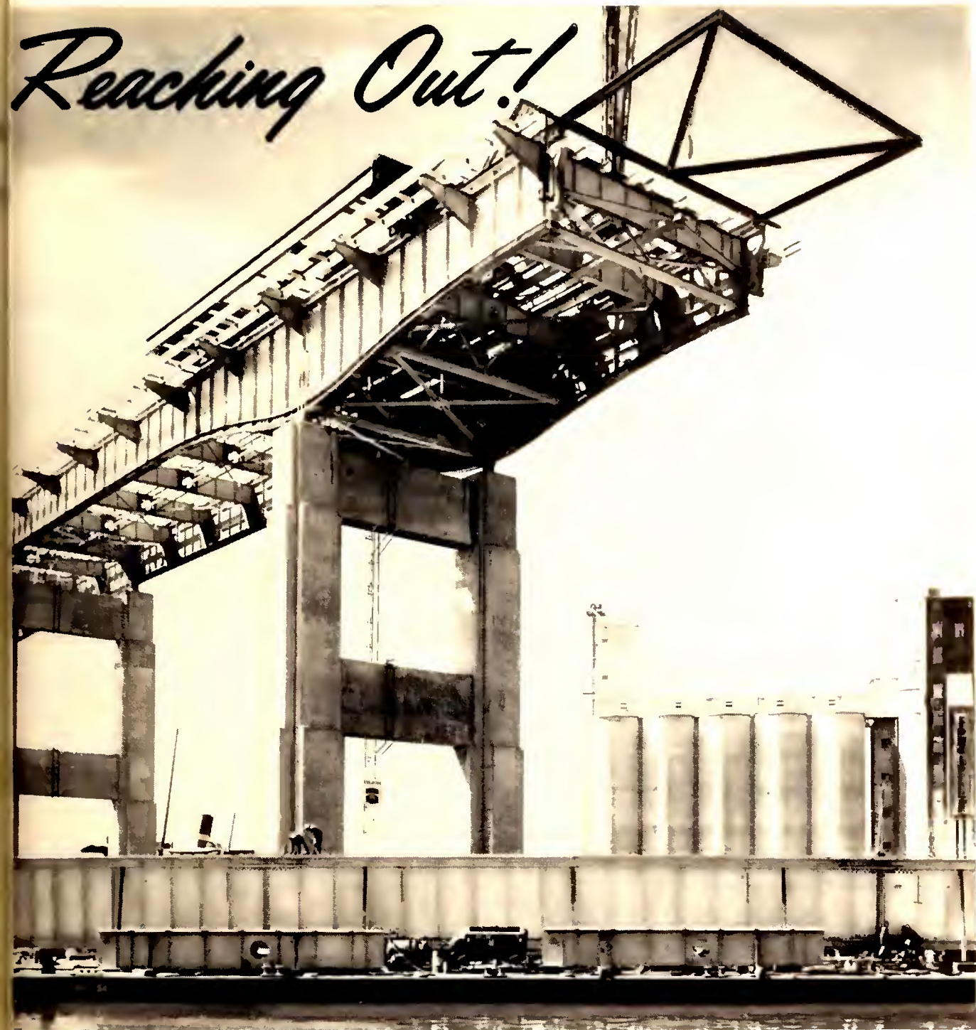
Hi-level bridge construction over Buffalo River
