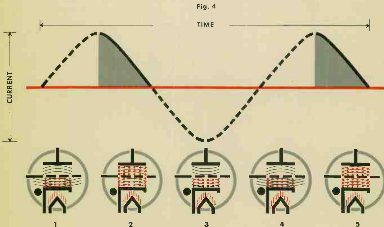
THE GRID ACTION OF A GAS-FILLED TUBE —1. Grid prevents flow of electrons—completely cancels effect of anode. 2. When less than a minimum voltage is applied to grid, full flow of electrons is suddenly released. 3. Anode is negative and does not attract electrons. 4-5. Cycle repeats.
