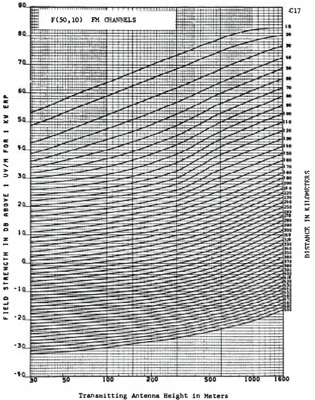
FCC 673.333 FIGURE 1a
