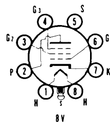
SYLVANIA TYPE 7A7 REMOTE CUTOFF RF PENTODE
