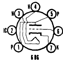
SYLVANIA TYPE 6C4 HIGH FREQUENCY POWER TRIODE
