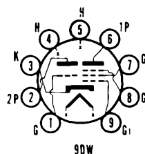
SYLVANIA TYPE 5AT8 TRIODE PENTODE
