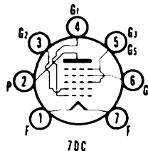
SYLVANIA TYPE 1L6 PENTAGRID CONVERTER
