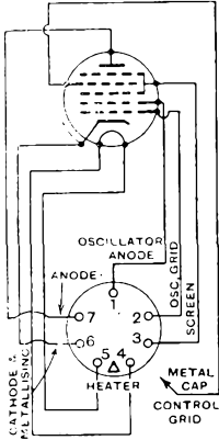
HEPTODES
