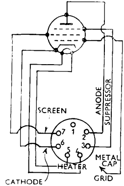
SCREEN PENTODES WITH GRID TOP CAP.
