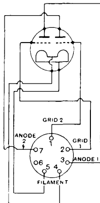
DOUBLE TRIODE "CLASS B"
