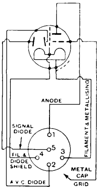
BATTERY DOUBLE DIODE-TRIODE
