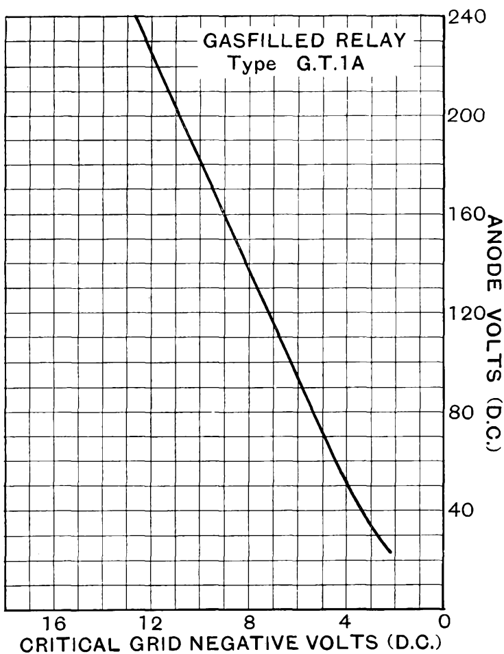
CHARACTERISTIC CURVE OF AVERAGE VALVE.
