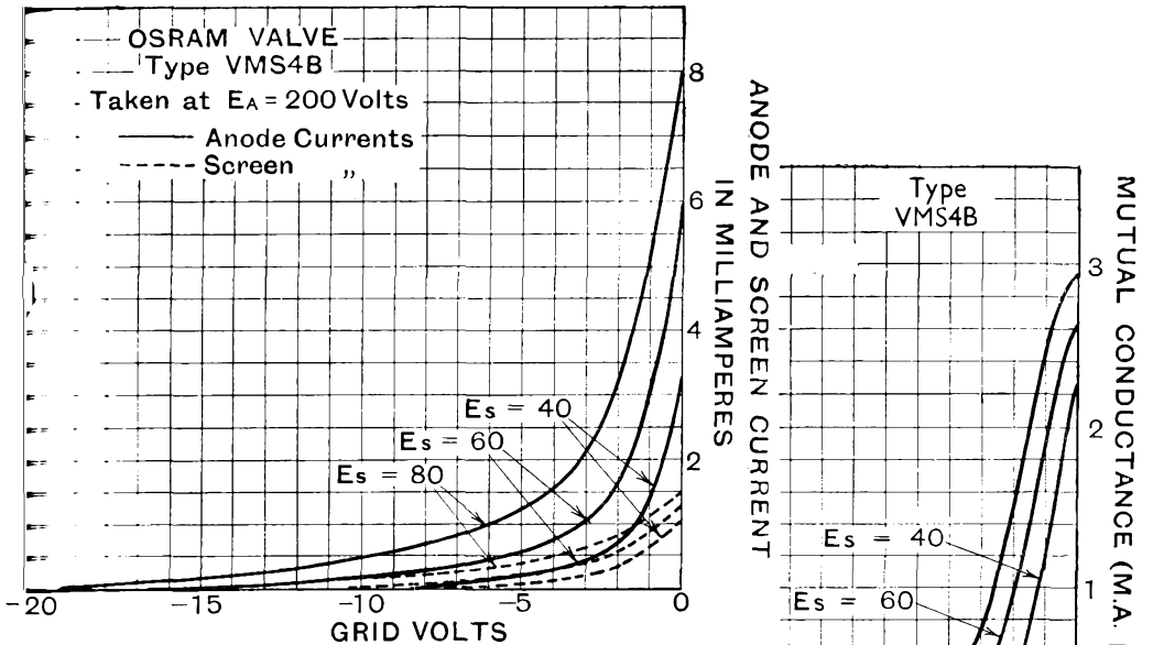
CHARACTERISTIC CURVES AVERAGE VALVES.
