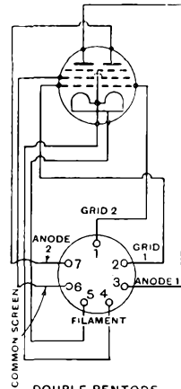
DOUBLE PENTODE
