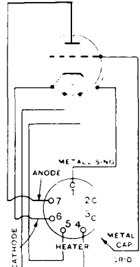
TRIODES WITH GRID TOP CAP.
