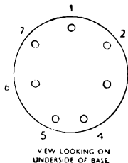
VIEW LOOKING ON UNDERSIDE OF BASE
