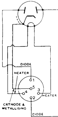
DOUBLE DIODE D41
