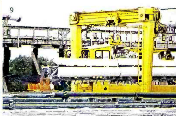
(9) High-rise crane truck, shown conveying special UHF Panel antenna to testing site, is typical of many special equipments employed in this unique antenna engineering site. Pylons in foreground await shipment.
