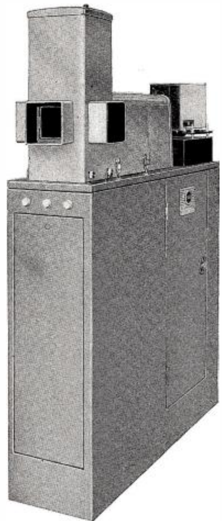
Type PF-11-A Pneumatic Multiplexer is manufactured for General Electric by Eastman Kodak Company to relay the optimum image from film and slide projectors to the vidicon camera. Pneumatically operated high efficiency front surface mirrors travel in their own plane and normal to the optical axis. This unique mirror mechanism and a very rugged base cabinet result in a stable and accurate relay system. The mirror switching system can be controlled at the unit or from remote operating positions.
