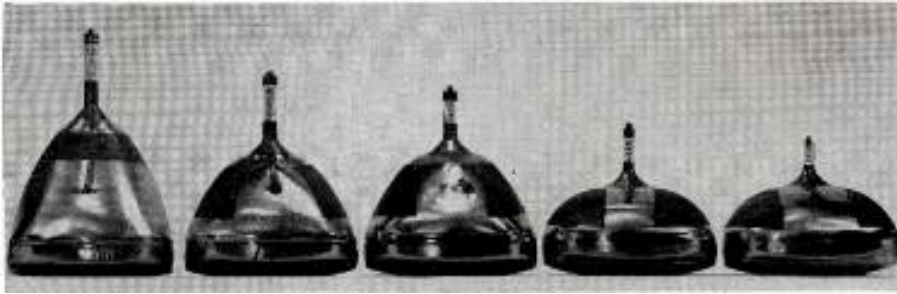
EVOLUTION of Philco's new "SF" (Special Form) tv tube is illustrated (l to r) by the 70-degree deflection tube (1950), two 90-degree tubes (1955 and 1956), the 110-degree tube (1957), and the SF Philco tube, described as the thinnest on the market this year. The SF tube is only 10 11/16 inches deep.
