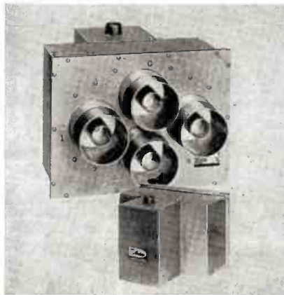
Andrew's remote control coaxial switch. Page 106
