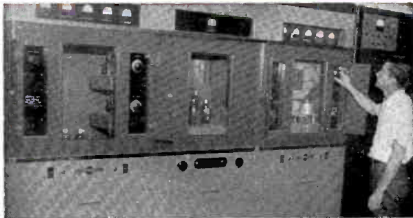
Collins 21E-5kw installation in KPHO's Radio transmitter building
