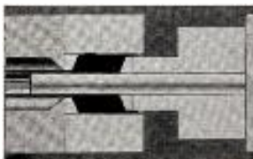
4) Outer ram pressure on billet is increased, forcing the metal through the opening between the inner ram and the die, forming the tube.
