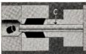
3) Inner ram "C" pierces billet and projects through the die, ejecting part of the metal displaced.
