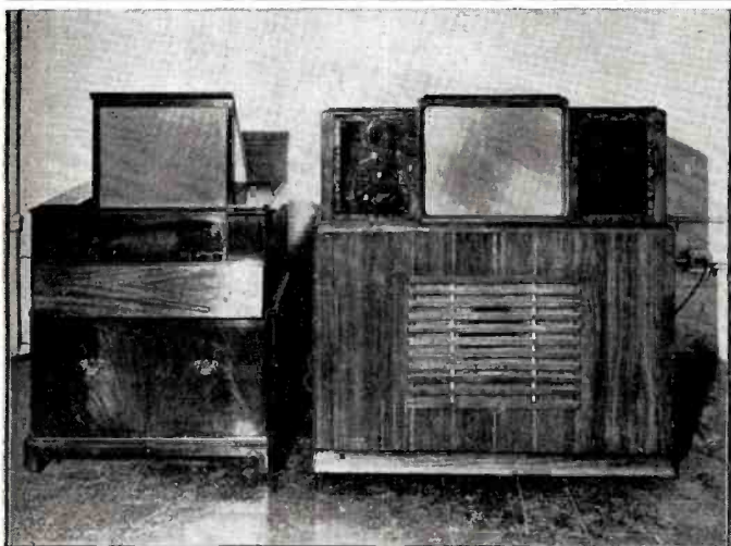
COLOR set (r) of Color Television Inc., alongside a black and white projection receiver.
