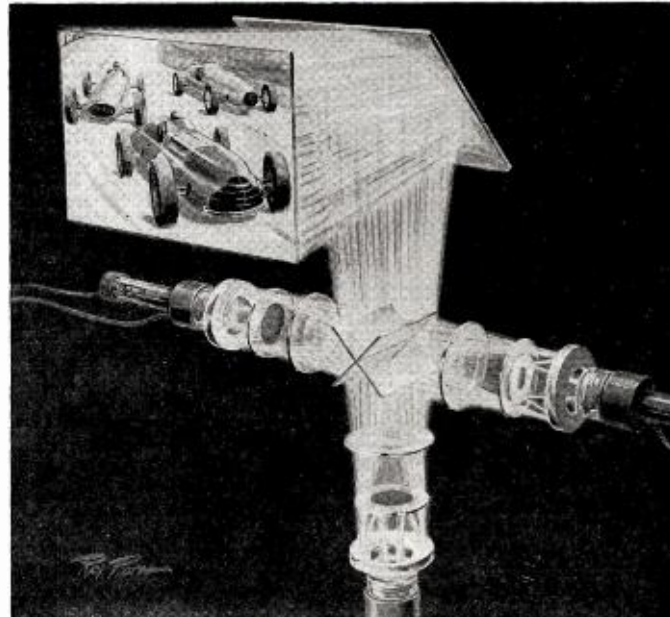
DIAGRAM of RCA's color television projection picture-reproducing system, using three projection kinescopes, reflective optics and a pair of dichroic mirrors. The kinescopes direct primary colors, after unscrambling color signal, onto the viewing screen via a refractive optical system. Each projection is of a different color—red, blue and green—which combine into a full color picture.
