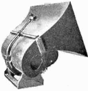
1926. Folded exponential horn used with the first sound motion pictures, developed hitherto unmatched volume.
