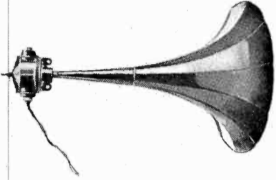
1921. Western Electric "morning glory" horn of the type used at the dedication of the Tomb of the Unknown Soldier in Arlington.
