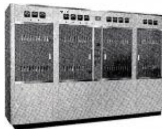
AM BROADCAST TRANSMITTERS, BTA-5H, 5 KW and BTA-10H, 10 KW. Lowest operating cost for tubes and power. Fewer tubes, fewer tube types to stock. Famous long-life RCA 5762's used in Modulator and P.A. Bi-level modulation assures wide-range frequency response—lowest distortion. Many other features . . . split-cycle overload protection, sliding doors, maximum component accessibility, simple two-tuning-control operation. Space saving floor plan.
