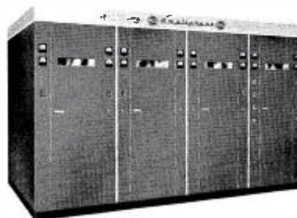
THE "AMPLIPHASE" 50 KW AM BROADCAST TRANSMITTER, BTA-50G Requires less than 80 sq. ft. of floor space—smaller than many 5 KW's. Internal ducts—no air duct installations necessary. Half the tube cost and lowest operating cost ever offered in a 50 KW transmitter. Long-life 5671 tubes used. Excellent frequency response and distortion characteristics. Permits remote-control or attended operation.
