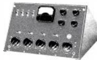
THE "BLOCK-BUILDER" AUDIO CONSOLE, BC-5A. Nine Inputs—4 microphones, 2 turntables, 2 remote lines, 1 network or tape. 4 mixer positions. Built-in power supply. Easily expanded for dual channel use by "pairing."
