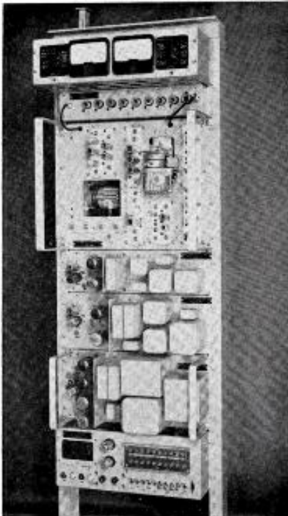
TYPE CE-900 MICROWAVE CARRIER TELEPHONE SYSTEM
