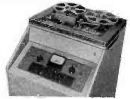
PRESTO SR-11 STUDIO TAPE RECORDER
