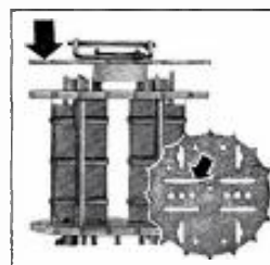
DOUBLE PLATE-TO-GRIOD LEAKAGE PROTECTION in many 5-Star types! Left: getter flash shield wards off conductive deposits. Right: spacer slots interrupt leakage paths.
