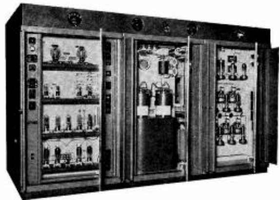
TYPE 315 and 316 5,000 WATT AM TRANSMITTER
