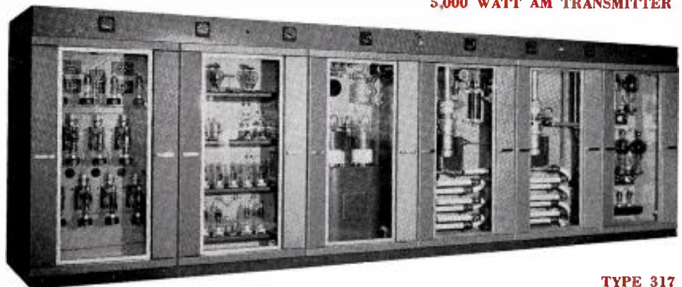
TYPE 317 50,000 WATT AM TRANSMITTER
