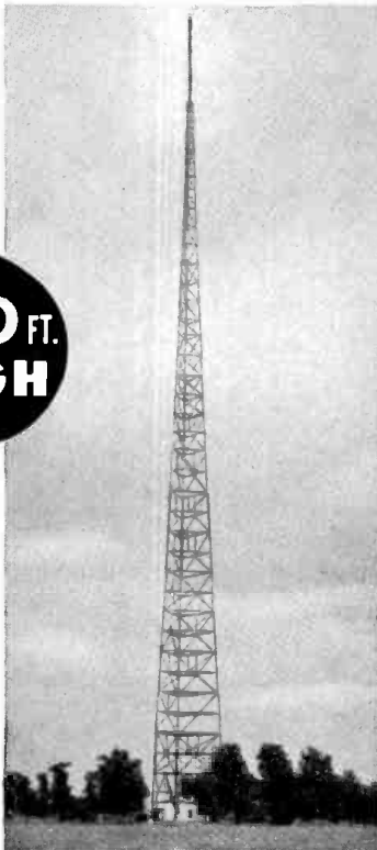
Below: KFAM, St. Cloud, Minn.— 440-foot Truscon Type H-30 Self-Supporting Radio Tower mounts an RCA 4-section FM Pylon. Overall height is 494 feet.
