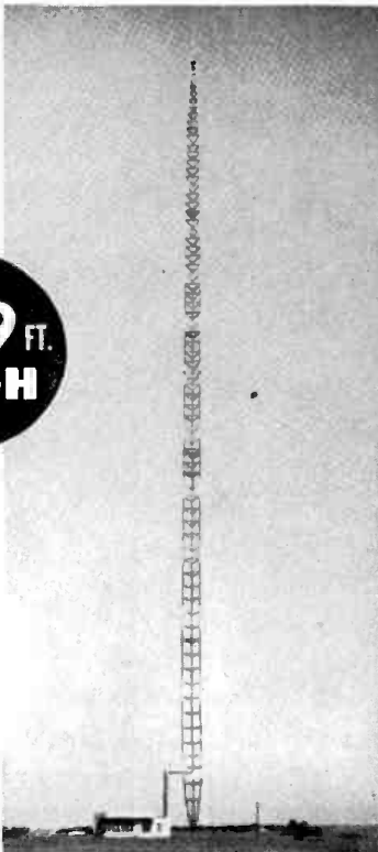
Below: This guyed Truscon Steel Radio Tower operated by KOCY, Oklahoma City, Okla., is 849 feet above ground, 938 feet high overall to top of General Electric FM antenna.
