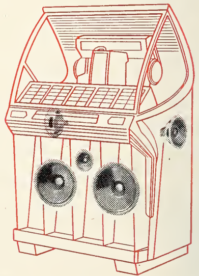
Mounted at the front of the acoustical chamber are two heavy-duty, 12-inch low-frequency speakers and a 5-inch high-frequency speaker. Wide-range 8-inch speakers are mounted on either side.
