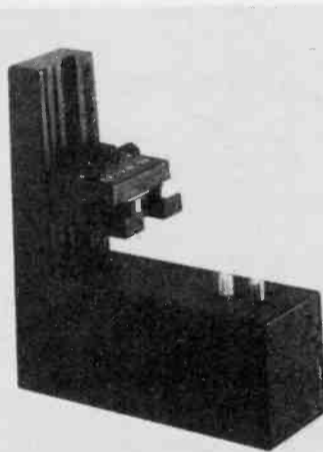
SPECIAL HEAD of magni-crystal ferrite is one of the meticulously crafted elements in the hand assembled Sansui stereo cassette deck model SC 363. Four-pole hysteresis synchronous drive motor and safety devices to prevent tape jamming, breakage, stretching, or accidental erasure are also featured. Photoelectric sensor shuts tape off automatically. Suggested list: $279.
