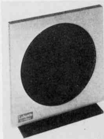
TRANSDUCER TWEETER with a flat diaphragm design by Lafayette, model RP-1000, in 4½ inch brushed aluminum case, can be internally mounted or freestanding. Etched voice coil is mounted in a super high energy rare earth samarium cobalt magnet structure. Suggested list: $59.95.
