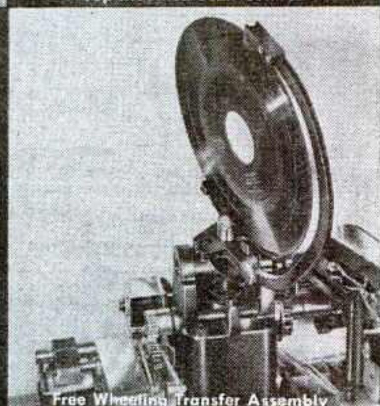
Free Wheeling Transfer Assembly
